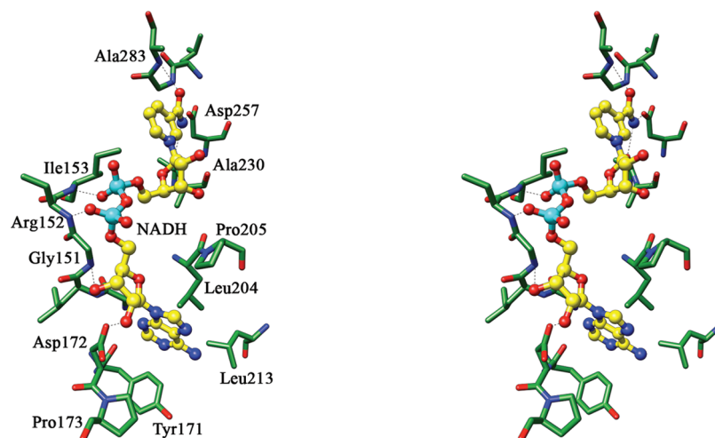
FIGURE 4: The cofactor binding site of chain B of M.tb PGDH with cofactor modeled into the site. A stereodiagram of the interactions of cofactor modeled into the cofactor binding site of chain B of M.tb PGDH is shown. The cofactor is shown in ball and stick representation with carbon atoms in yellow, nitrogen atoms in blue, oxygen atoms in red, and phosphorus atoms in cyan. The protein is shown in green. All hydrogen bonds, represented as dashed lines, are within the distance of 3.5 Å. In this figure, the side chain of Arg152 has been truncated in order to prepare this stereo representation.
