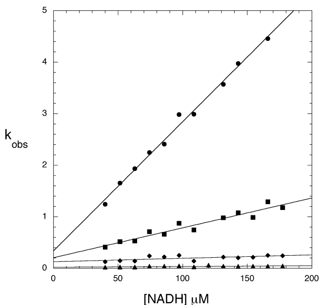
FIGURE 8: Plot of k_{\text{obs}} vs NADH concentration. The binding of NADH to M.tb PGDH was investigated with pre-steady-state transient kinetic analysis. The observed rates obtained from fitting the pre-steady-state transients to an equation for four exponentials are plotted against the NADH concentration. Two concentration dependent ( \bullet , \blacksquare ) and two concentration independent ( \blacklozenge , \blacktriangle ) curves are fit to a straight line.
