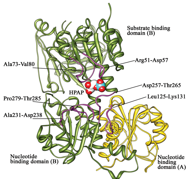
FIGURE 1: M.tb PGDH active site. The figure shows the loops bordering the active site of M.tb PGDH in chain B in purple. The active site is formed by both chains. The nucleotide and substrate binding domain of chain B are shown in dark green. The intervening and regulatory domains are not shown for clarity. The nucleotide binding domain of chain A is in gold. The substrate, HPAP, is shown in space filling representation bound at the active site (carbon atoms are white, oxygen atoms are red, and phosphorus is cyan).
