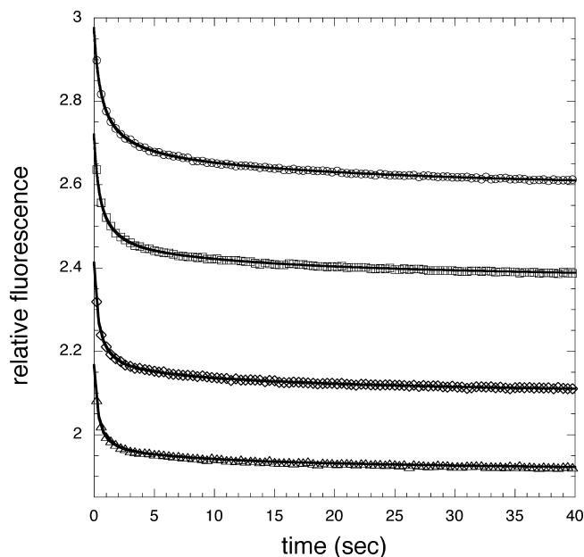
FIGURE 7: Pre-steady-state transients from the binding of NADH to M.tb PGDH. The figure shows representative presteady state transients produced by the binding of NADH to the enzyme. The relative change in fluorescence of tryptophan upon binding of NADH is depicted by the symbols. The sample was excited at 295 nm and the fluorescence at 340 nm was recorded after rapid mixing of enzyme and NADH. Four representative transients are shown for 86 \mu\text{M} ( \circ ), 109 \mu\text{M} ( \square ), 143 \mu\text{M} ( \diamond ), and 167 \mu\text{M} ( \triangle ) NADH. The enzyme concentration was 2 \mu\text{M} in subunits. Only every 100th point is shown for clarity. The solid lines are the fits to the data using eq 3 for 4 exponentials. The binding exponentials are essentially complete within 2 s. The remaining two exponentials represent a slow conformational change over the 2–40 s range shown.
