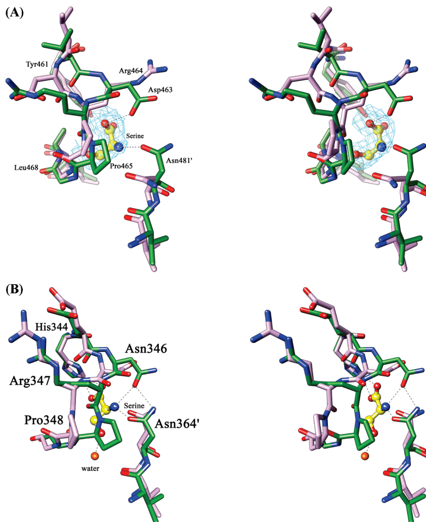
FIGURE 9: Stereoview of the changes occurring at the allosteric site upon serine binding. (A) In M.tb PGDH, superimposition of the regulatory domain of chain A of the apo-enzyme (purple) and the serine bound form (green) shows a flip of the side chains of Asp463 and Arg464, present on the loop region lining the allosteric site. Also seen is the change in orientation of Asn481' from the adjacent subunit, which covers the allosteric site upon serine binding. Serine is depicted in yellow ball and stick. The Shake&wARP unbiased 2F_o - F_c electron density map of serine is shown in light blue ( 1\sigma level contour). (B) In E. coli PGDH, superimposition of the regulatory domain of chain A of the apo-form (purple) with the serine inhibited form (green) shows a transition of the loop region at Pro348, without side-chain flipping. In this case, transition of the Pro348 covers the allosteric site upon serine binding. Serine is shown at this site in the form of ball and stick (yellow). In both figures, the hydrogen bond interactions of serine with the protein are shown as dashed lines, oxygen atoms are shown in red, and nitrogen atoms in blue.
