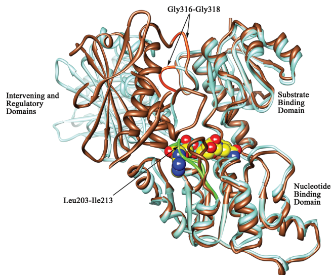
FIGURE 6: Orientation of the loop region at the cofactor binding site and the strand connecting the substrate binding domain to the intervening domain. A ribbon diagram representation of the superimposition of chain A (in brown) on chain B (in aquamarine) showing the orientation of the loop region (residues 203–213 designated with arrows) at the cofactor binding site in the M.tb PGDH structures and the glycine containing strand (residues 316–318) connecting the substrate binding and intervening domains. The NADH molecule is represented in space filling representation (carbon atoms are in yellow, oxygen atoms are in red, nitrogen atoms are in blue, and phosphorus atoms are in aquamarine) and has been modeled into this site based on the E. coli PGDH structure. This figure depicts the loop movement near the cofactor binding site in both chains. As shown with an arrow, the loop region in chain B (green) falls over the cofactor binding site, thus blocking NADH from binding at this site in these crystal structures. Also apparent in this figure is the change in the domain orientation of the intervening domain-regulatory domain unit. A portion of the regulatory domain in chain A has been clipped in the front for clarity. The location of Gly316-Gly318 is shown in orange in the loop connecting the substrate binding and intervening domains.
