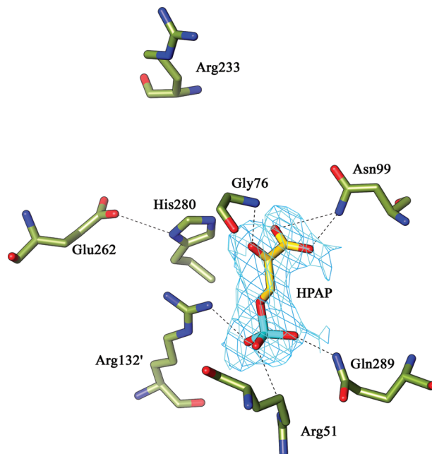
FIGURE 2: Interaction of HPAP at the M.tb PGDH active site. This figure shows all the residues involved in the HPAP interaction in chain B of the substrate bound M.tb PGDH structure. Also shown are the catalytic dyad His280:Glu262 and Arg233 in relation to HPAP at the active site. The Shake&wARP unbiased 2F_o - F_c electron density map for HPAP (light blue) is contoured at the 1\sigma level. HPAP is shown within the electron density. Oxygen atoms are shown in red, nitrogen atoms are in blue, and phosphorus atoms are in cyan.
