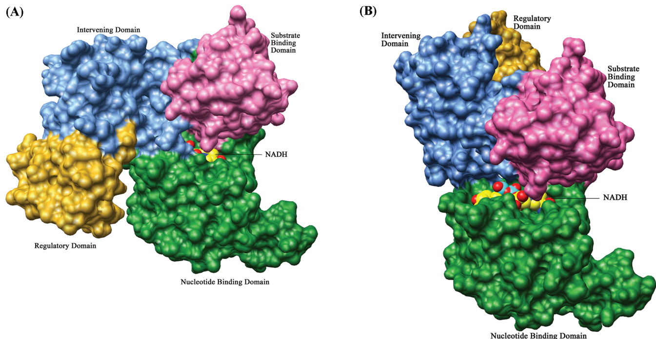
FIGURE 5: Modeling of NADH binding to the cofactor binding sites in Chain A and Chain B. Molecular surface representations of M.tb PGDH chains showing the two different cofactor binding sites. In both chains, the four domains are represented with different colors: nucleotide binding domain (green), substrate binding domain (pink), intervening domain (blue) and the regulatory domain (yellow). NADH has been modeled in both figures in space filling representation (carbon atoms are in yellow, oxygen atoms are in red, nitrogen atoms are in blue, and phosphorus atoms are in aquamarine). The nucleotide (green) and substrate binding (pink) domains are orientated in the same way in both figures. (A) In chain A, the cofactor binding site resides in a channel which is formed by the intervening domain (blue) and nucleotide binding domain (green). (B) In chain B, the loop (see Figure 4), which blocks the cofactor binding site in these structures, has been placed similar to chain A. As seen in this figure, this site is now totally exposed to the solvent as the intervening domain (blue) is oriented away from the binding site.
