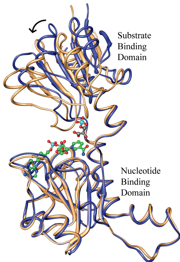
FIGURE 3: Model for the active site closure of M.tb PGDH upon substrate binding. A ribbon diagram of the M.tb apoenzyme (blue) is superimposed on a modeled ribbon diagram of M.tb PGDH (gold) based on the malate and NAD bound human PGDH structure (pdb code 2G76). NADH (green) and HPAP (gray) are shown in ball and stick form. As seen in the figure, there is a rotation of approximately 15° (arrow) of the substrate binding domain in response to substrate and cofactor binding. The intervening domain and the regulatory domain are not shown for the sake of clarity.
